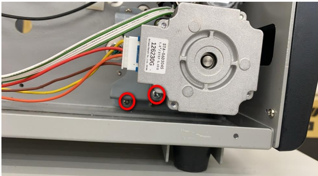
FIG 2. Remove 2 screws on the motor and motor bracket (red circles marked)
