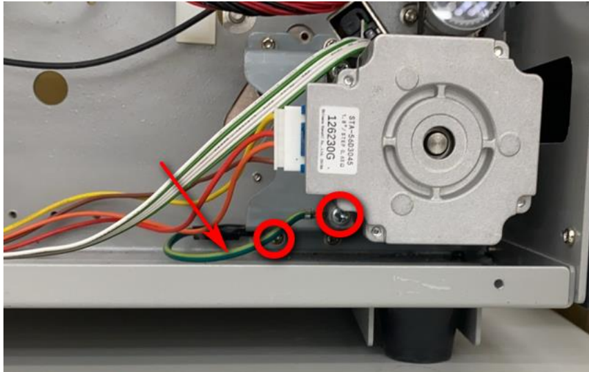
FIG 3. Fasten the screw on the motor side with the ground cable and the other side on the motor bracket (red marks)
